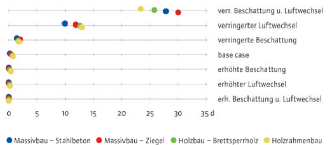
Simulation Innenraumtemperatur [7.12]
